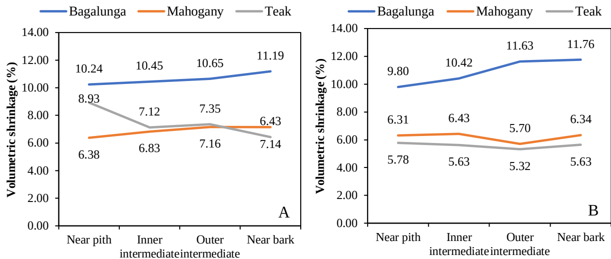
Fig. 8. Radial variation in the volumetric shrinkage of the three species: (A) butt and (B) middle portions.
