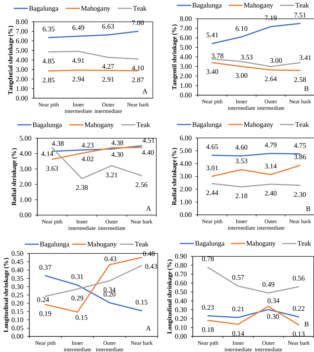
Fig. 7. Radial variation in directional shrinkage of the three species: (A) butt and (b) middle portions.
