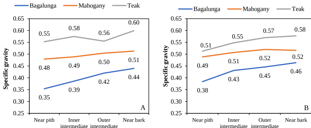
Fig. 6. Radial variation in specific gravity of the three species: (A) butt and (B) middle portions.
