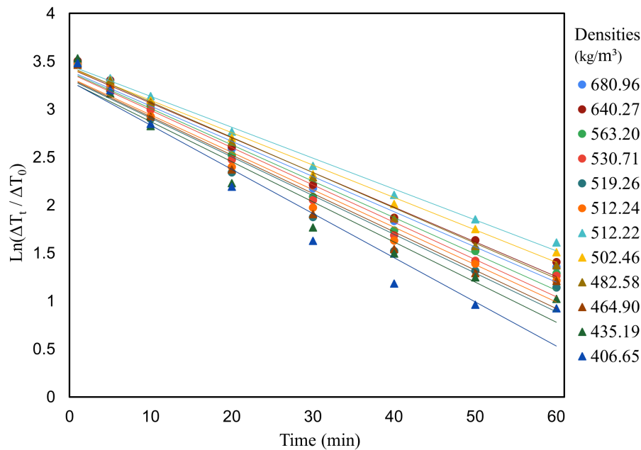
Fig. 3. Semi-logarithmic plots of \ln(\Delta T_t/\Delta T_0) versus time for mahogany (circles) and yemane (triangles). Near-linear trends indicate exponential cooling behavior, with shallower slopes in denser samples reflecting lower cooling rates.
